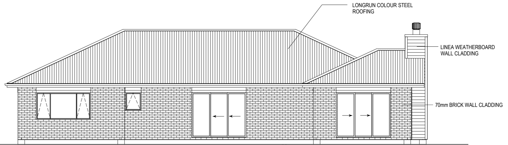
WEST ELEVATION
