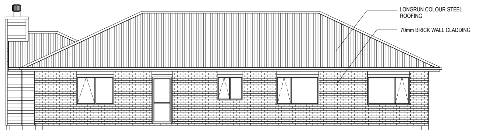
EAST ELEVATION
